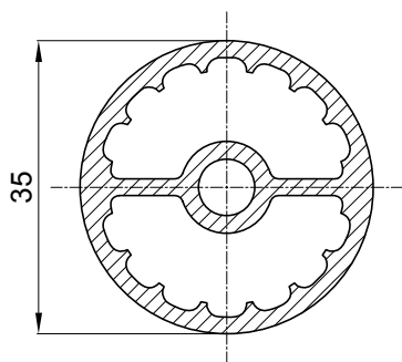
Profilo montante neutro Neutral upright profile
