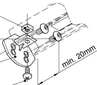
Kit staffa reggiplafoniera compl. Compl. light canopy bracket kit
