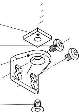
Kit staffa reggiplafoniera completo Complete light canopy bracket kit
