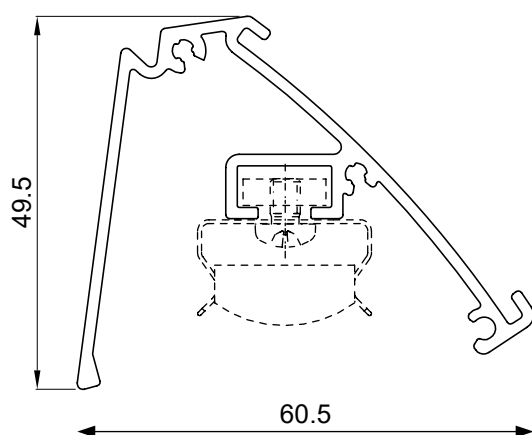
Profilo lampada Light canopy profile
