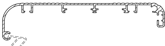
Profilo cappello Top shelf profile
