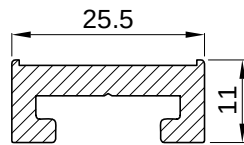
Profilo rotaia per mensola Key rail profile for shelf
