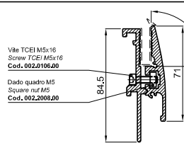
Profilo carter superiore (viti escl.) L=5000mm Cod. 150.7750
