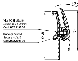
Vetro piano inclinato 10.5°
