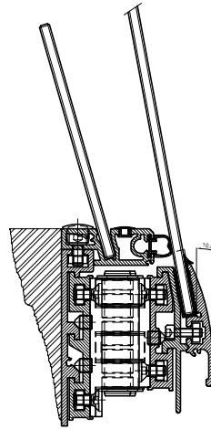
Vetro piano inclinato 10.5°
