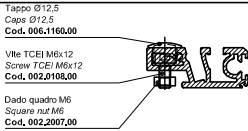
Profilo carter superiore (viti escl.) L=5000mm Cod. 150.7750
