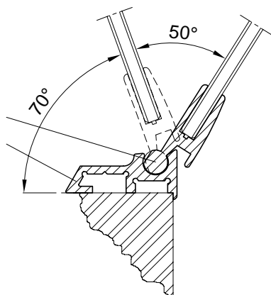
Profilo maniglia Hand grip profile
