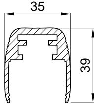
Profilo supporto Support profile
