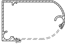
Profilo lampada Light canopy profile
