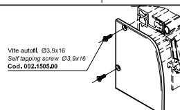
Complete end cap with screws Dx/Rt Sx/Lt* Cod. 150.1803 Cod. 150.1804
