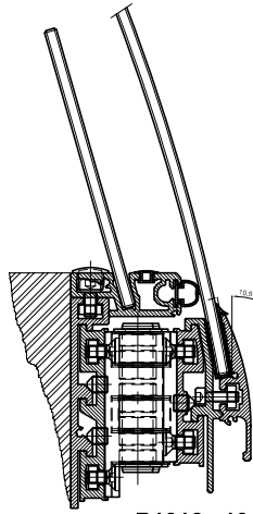
R1016 - 10.5° angle glass
