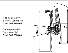
0° Complete hand grip 0° L=5000mm Cod. 150.8050
