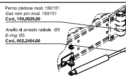
Gas spring for linear case complete kit 150N Cod. 150.0150.00 200N Cod. 150.0200.00
