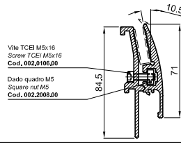
10.5° Complete hand grip 10.5° L=5000mm Cod. 150.7650
