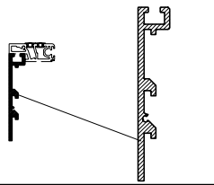
R1016 - 10.5° angle glass
