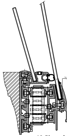
10.5° angle flat glass
